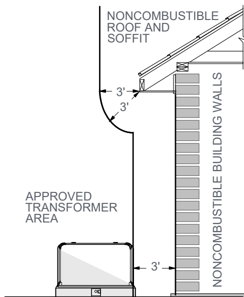
TRANSFORMER CLEARANCES FROM NONCOMBUSTIBLE SURFACES
