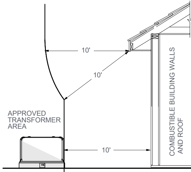
TRANSFORMER CLEARANCES FROM COMBUSTIBLE SURFACES
